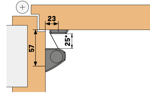
Mindestabstand/minimum distance/écart minimum
